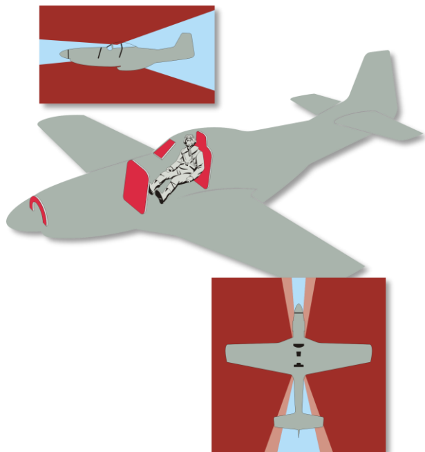
Figure 29: P-51D Armor
