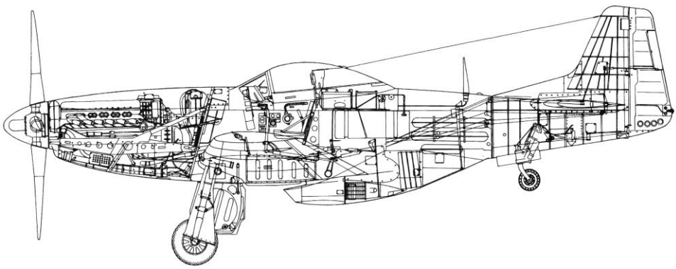
Figure 7: P-51D Fuselage
