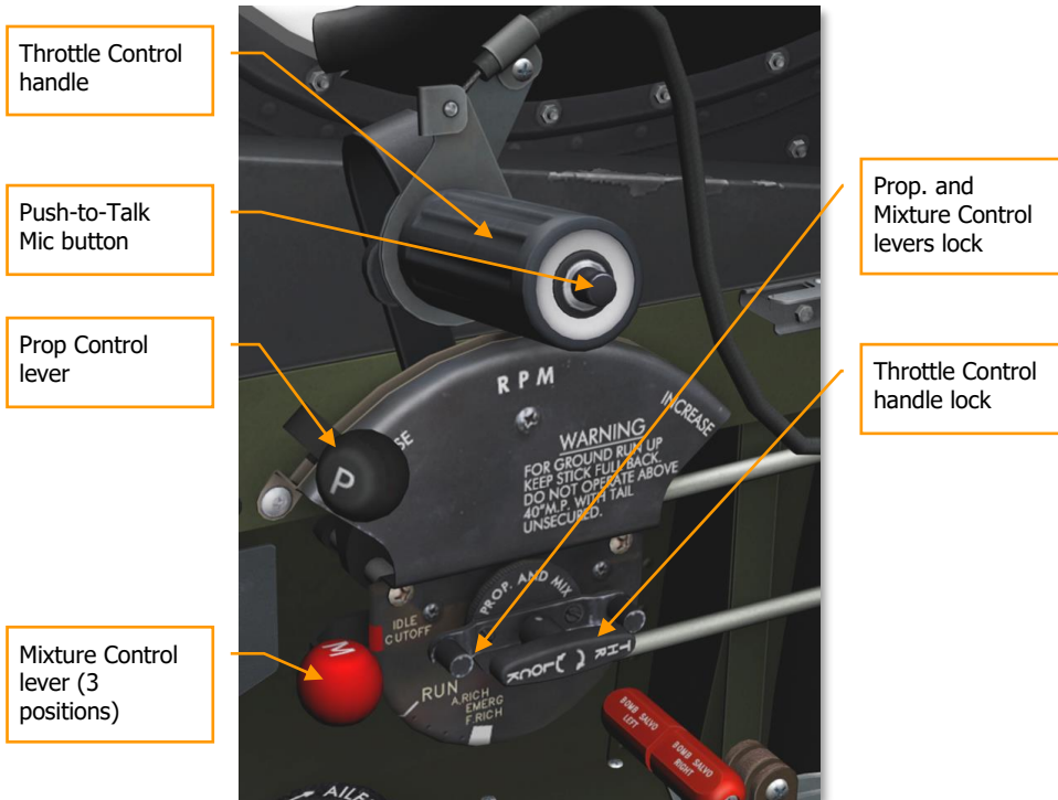
Figure 64: Throttle Quadrant
