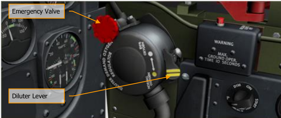
Figure 72: Oxygen Regulator
