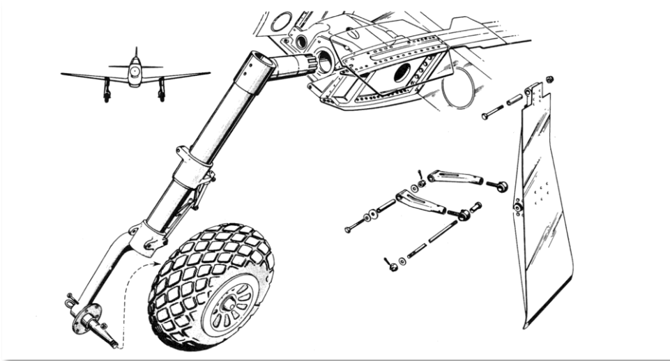
Figure 12: P-51 Main Landing Gear Housing, Fairing and Shock Strut
