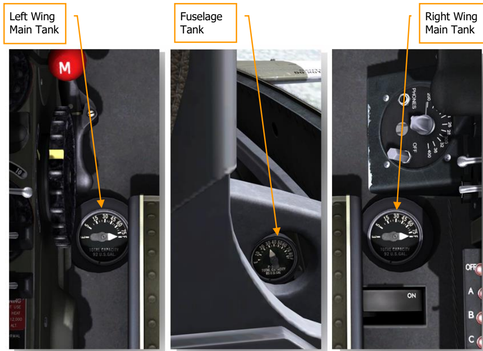
Figure 21: Fuel Gauges
