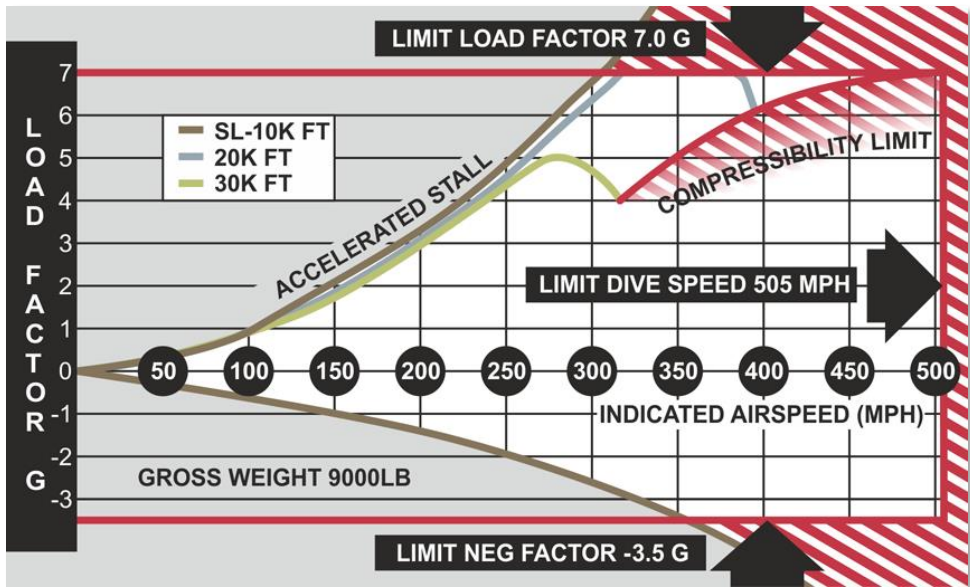
Figure 82: Load Factor Limitations
