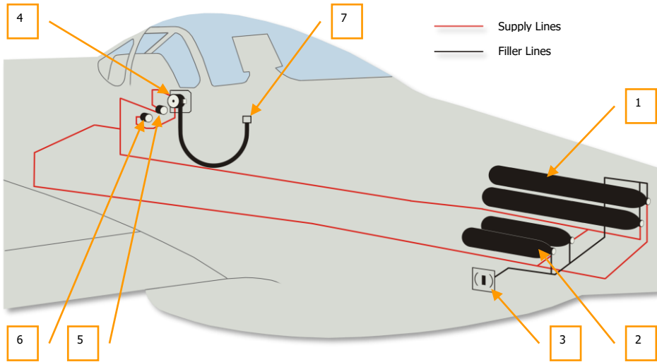
Figure 27: Oxygen System
