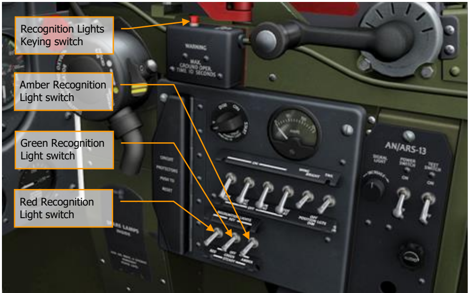
Figure 73: Recognition Lights
