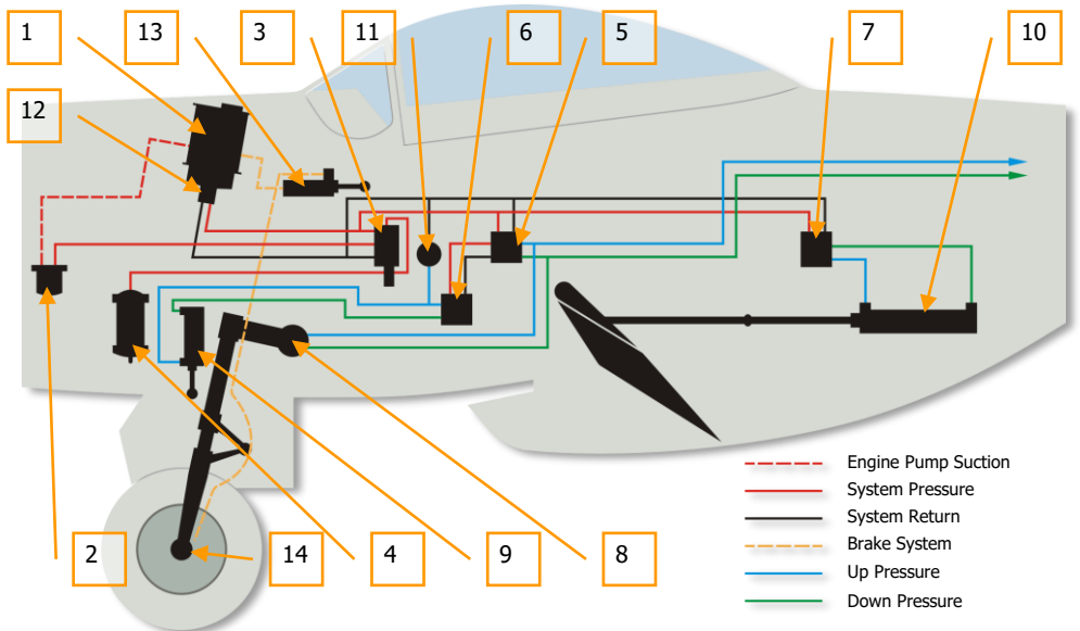
Figure 22: Hydraulic System
