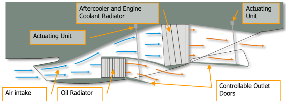
Figure 23: P-51D Radiators
